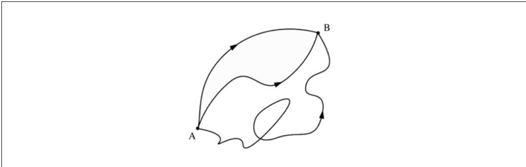
Figure 2: Quantum Paths
